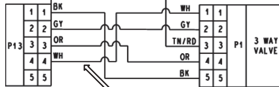
3 way refrigerant Valve
