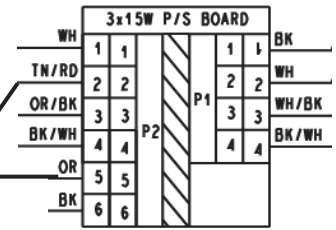
Power Supply Board
