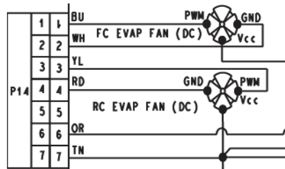
Control Circuit Board
